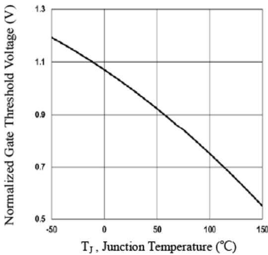
Fig.3 Normalized V_{GS(th)} vs T_J
