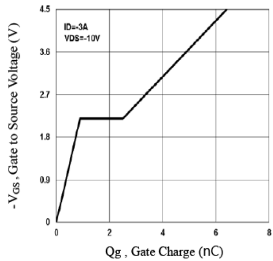
Fig.4 Gate Charge
