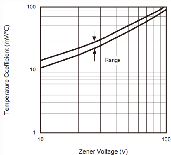
FIG.2 Temperature Coefficients vs. Zener Voltage
