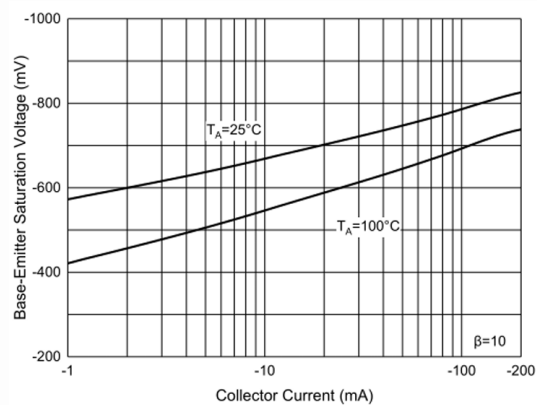
Figure 4. Base-Emitter Saturation Voltage Characteristics
