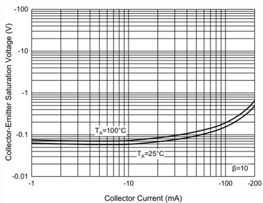
Figure 3. Collector-Emitter Saturation Voltage Characteristics
