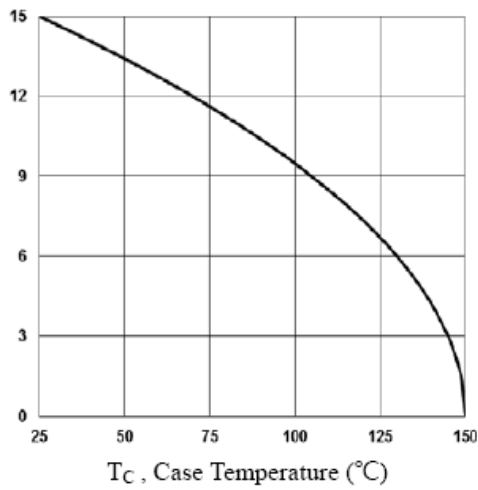
Fig.1 Continuous Drain Current vs. T_C
