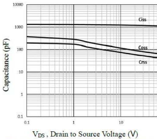
Fig.7 Capacitance Characteristics
