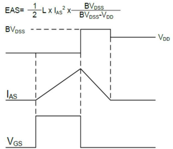
Fig.8 EAS Waveform
