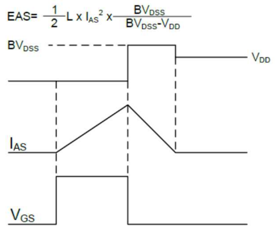
Fig.8 EAS Waveform
