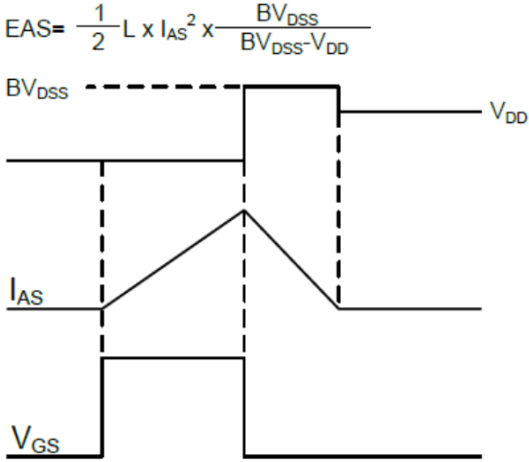
Fig.8 EAS Waveform
