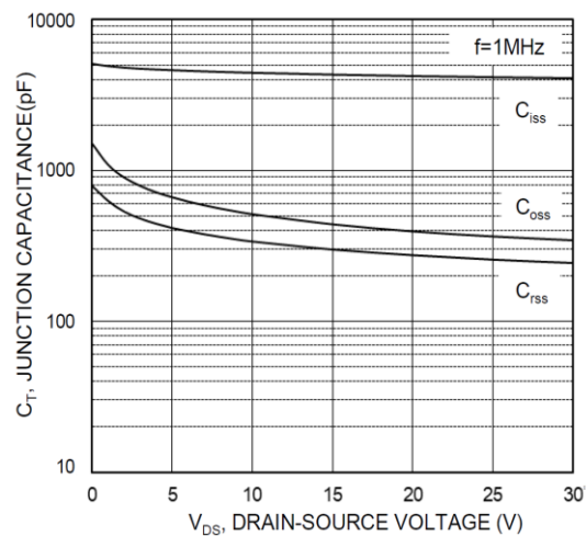
Figure 6. Capacitance
