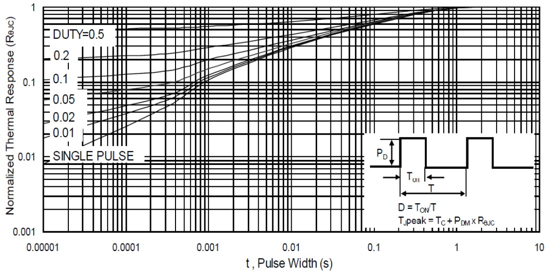
Figure 9. Normalized Transient Thermal Resistance
