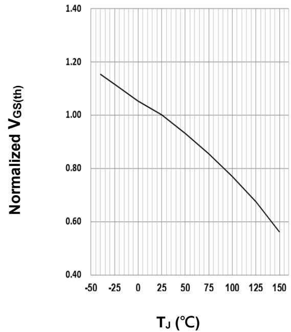
FIG.6 Normalized V_{GS(th)} vs. T_J
