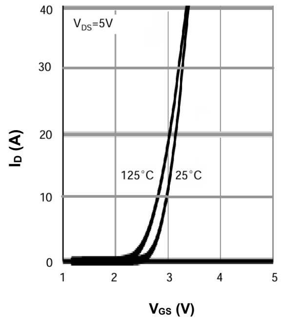
FIG.2 Transfer Characteristics
