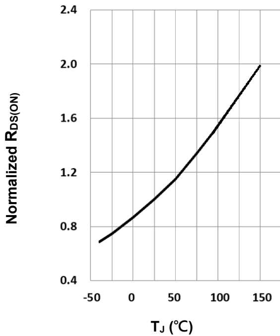
FIG.5 Normalized On-Resistance vs. T_J
