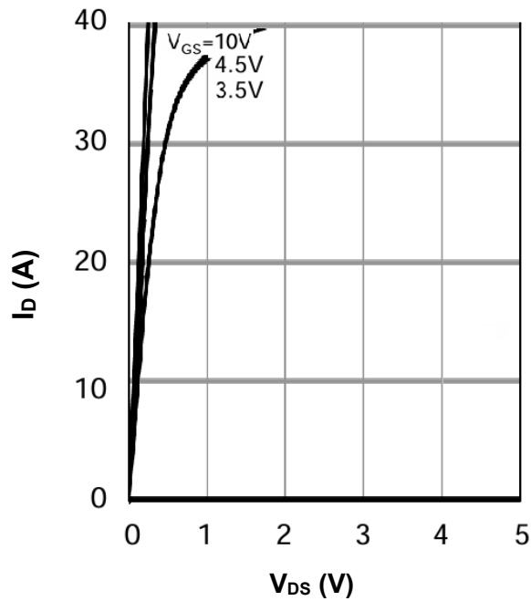
FIG.1 Output Characteristics
