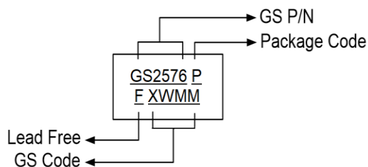
Adj Version
