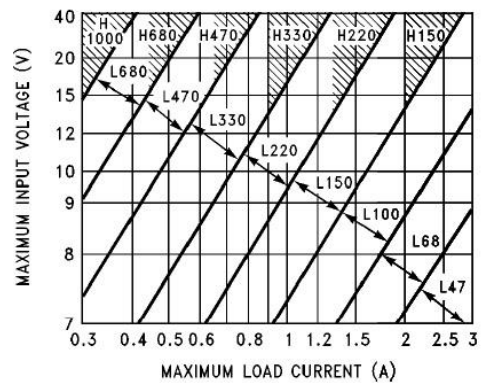
GS5276-50
