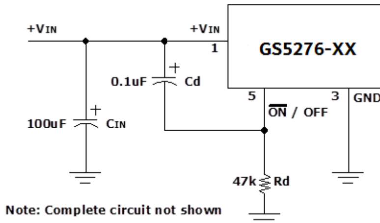
FIGURE 4. Delayed Startup
