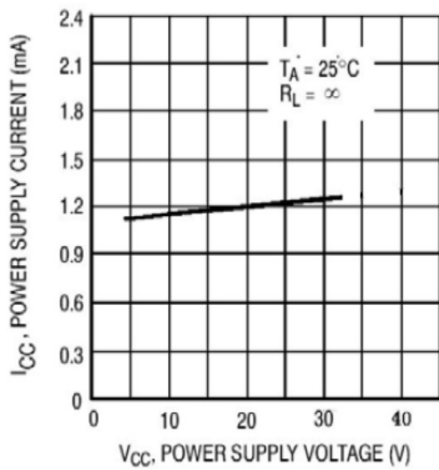
Supply Current
