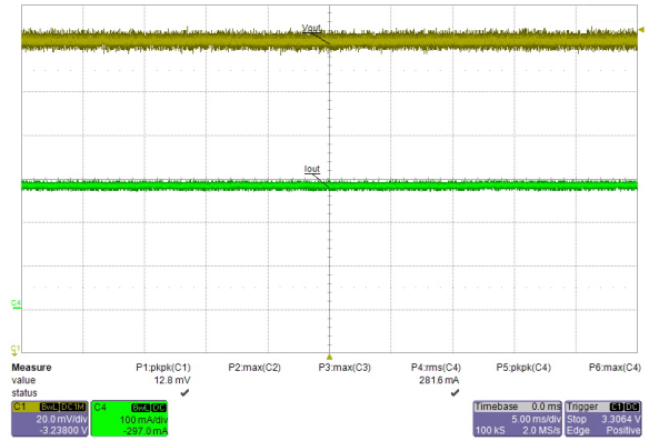
Fig 4. I_{OUT} = 300mA
