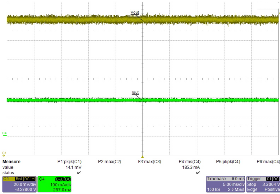
Fig 3. I_{OUT} = 200mA
