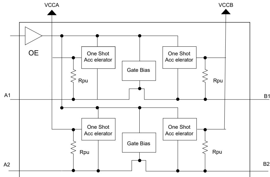
Figure 1: Block Diagram
