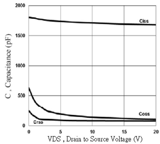
Fig.6 Capacitance Characteristics
