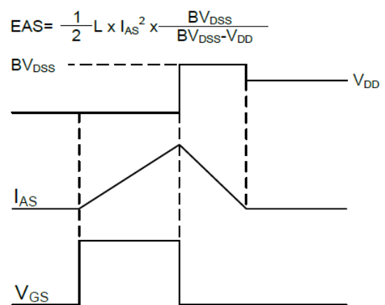
Fig.11 EAS Waveform
