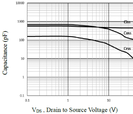
Fig.7 Capacitance Characteristics
