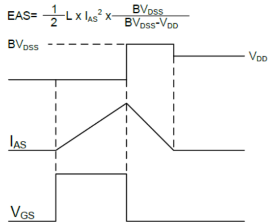
Fig.8 EAS Waveform
