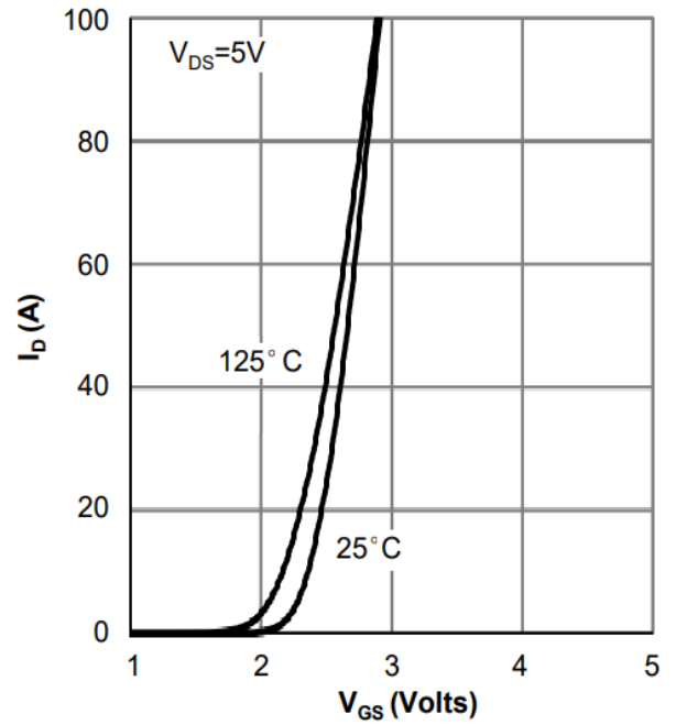
FIG.2 Transfer Characteristics
