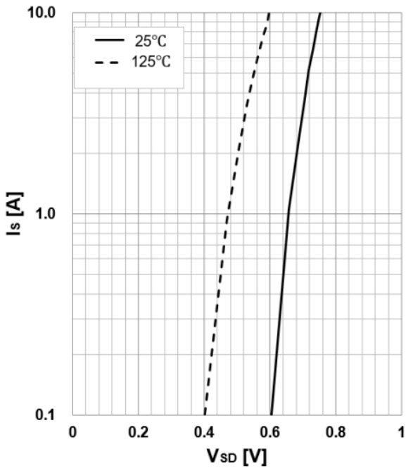
FIG.11 Body-Diode Characteristics
