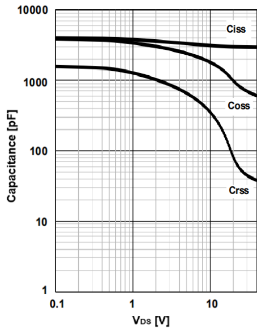
FIG.8 Capacitance Characteristics
