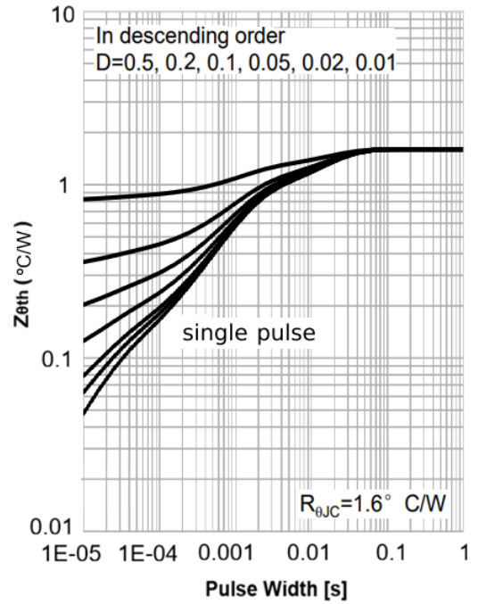
FIG.10 Transient Thermal Impedance
