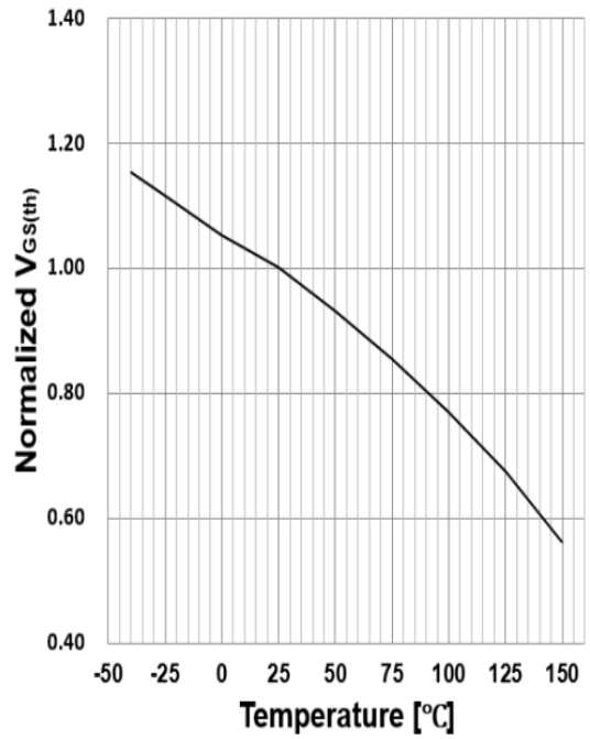
FIG.6 Normalized V_{GS(th)} vs. T_J
