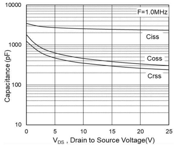
Fig.8 Capacitance Characteristics
