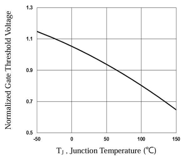
Fig.6 Normalized V_{GS(th)} vs. T_J
