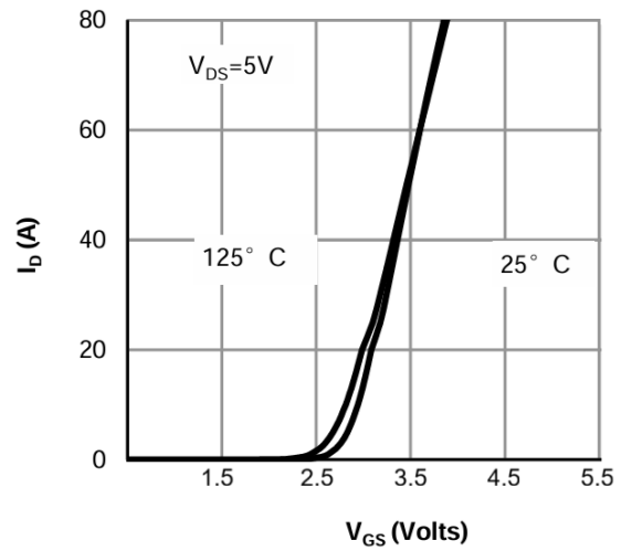
Fig.2 Transfer Characteristics
