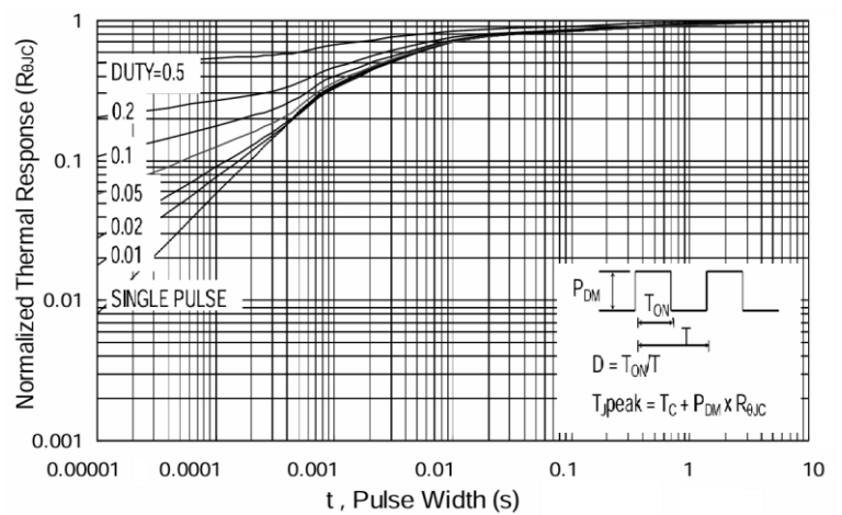
Fig.10 Normalized Transient Impedance
