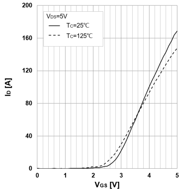
FIG.2 Transfer Characteristics
