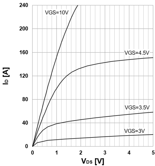
FIG.1 Output Characteristics
