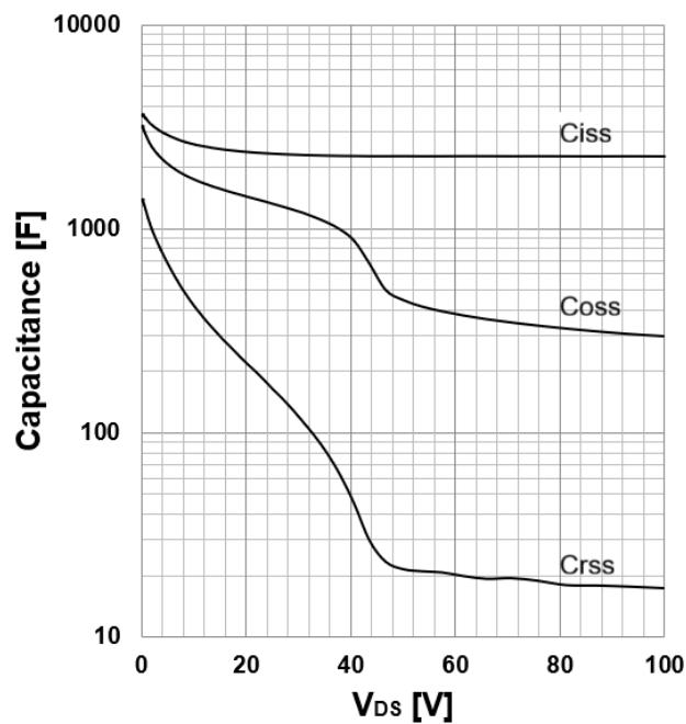
FIG.8 Capacitance Characteristics
